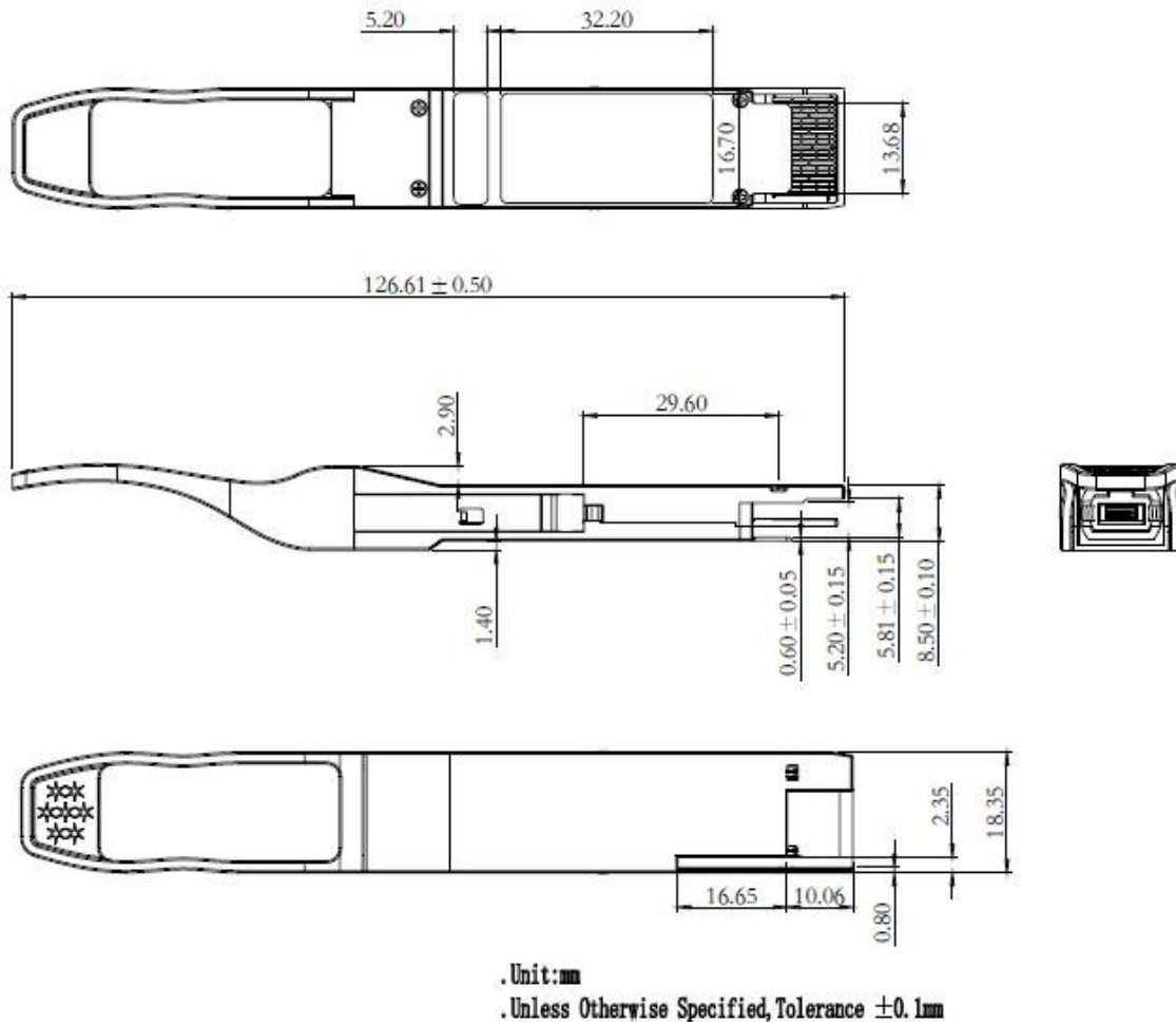
Figure10. Mechanical Specifications
