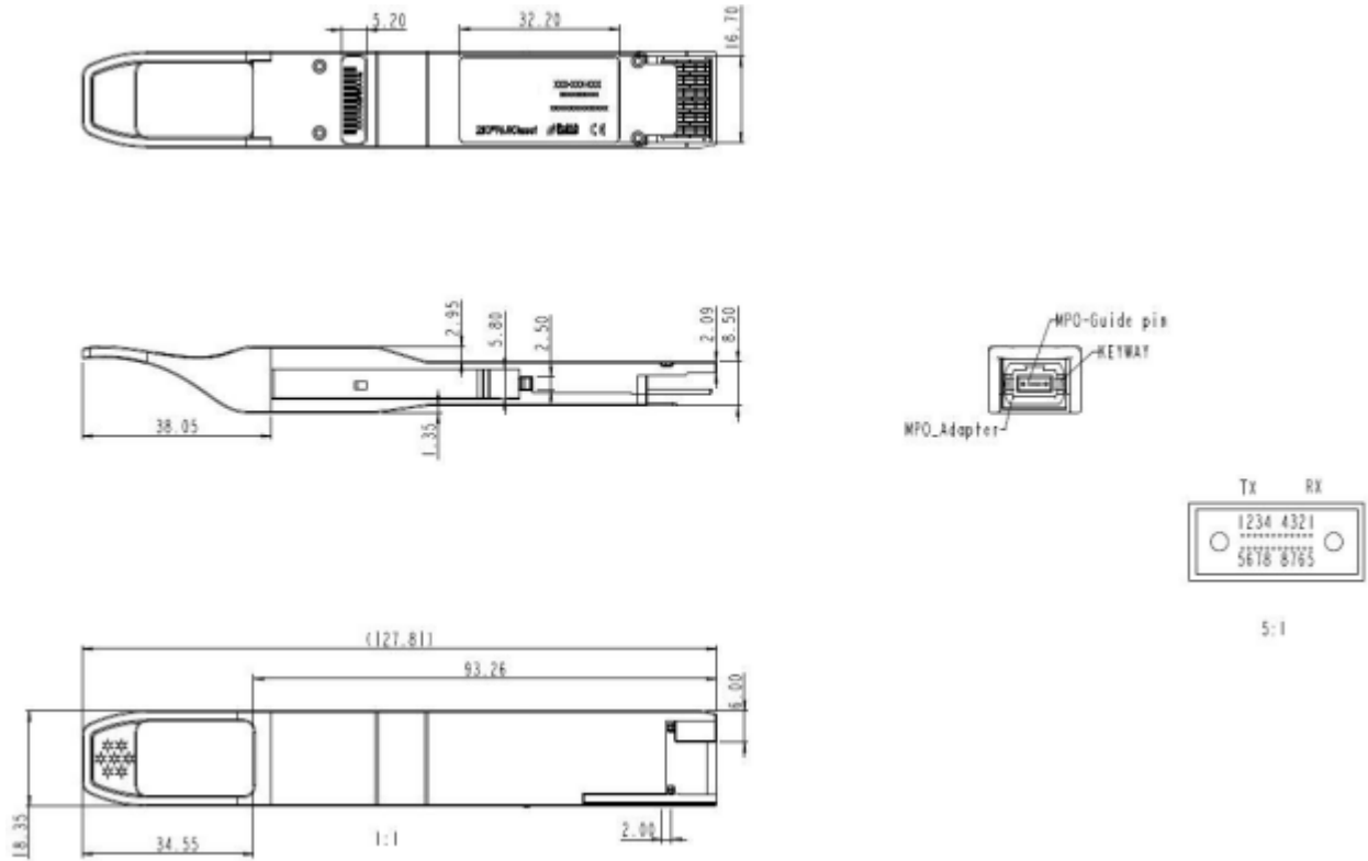
Figure6. Mechanical Specifications
